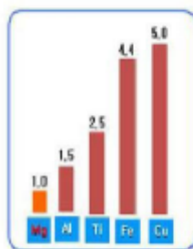
→ Weight Comparison
